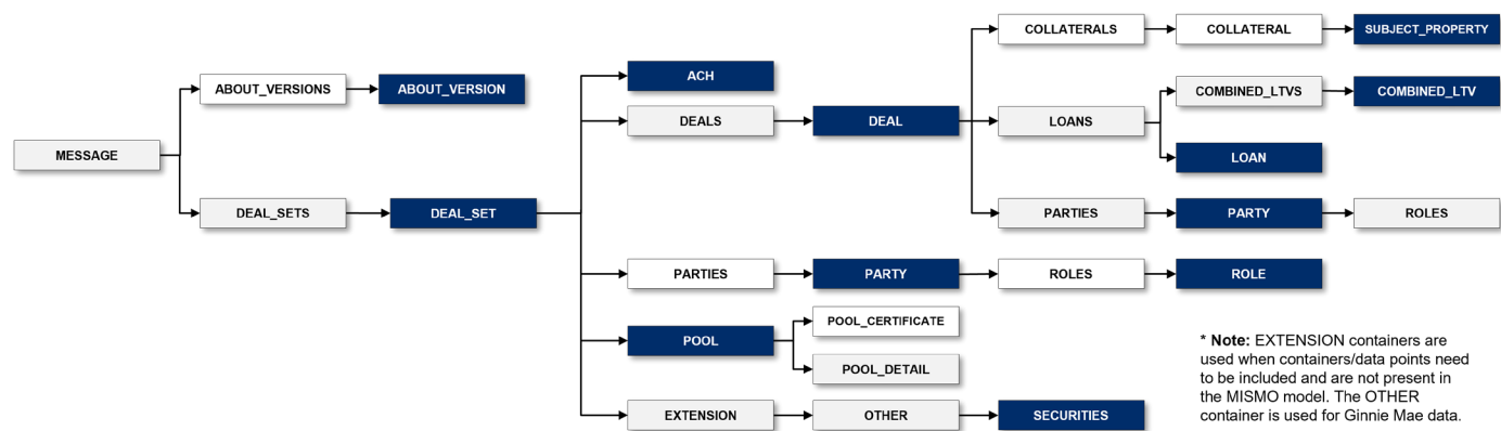
Figure 1: PDD High-Level Container Hierarchy
